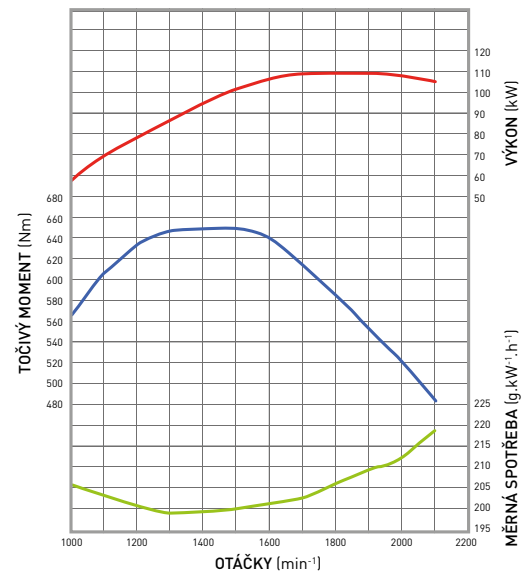
TCD 6.1 L6 – 106,1 kW
