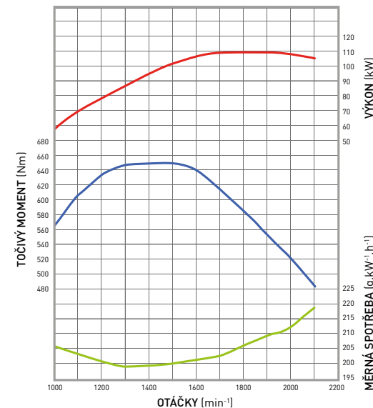
TCD 6.1 L6 – 120,1 kW
